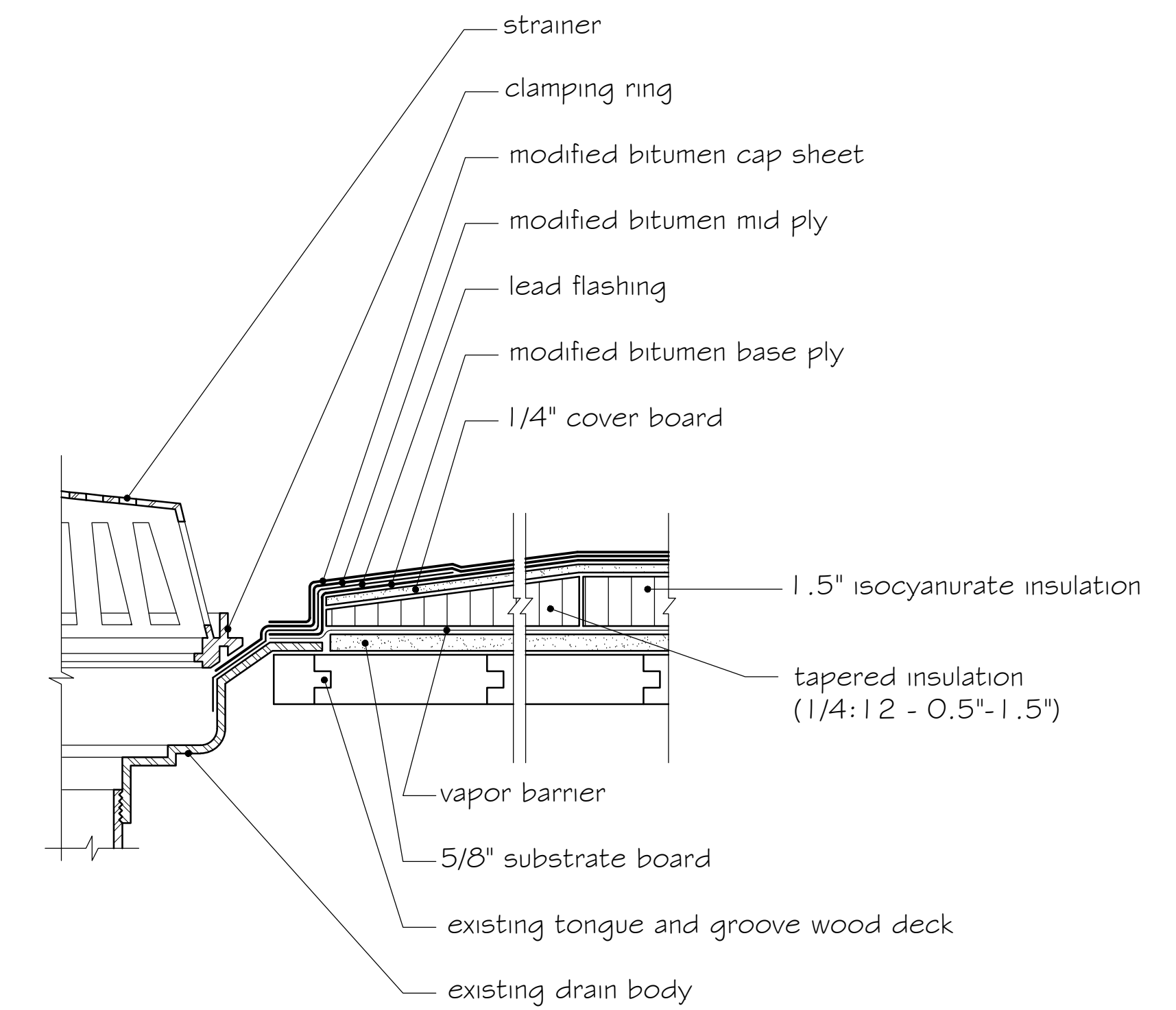
9 ROOF DRAIN - AREA 29
