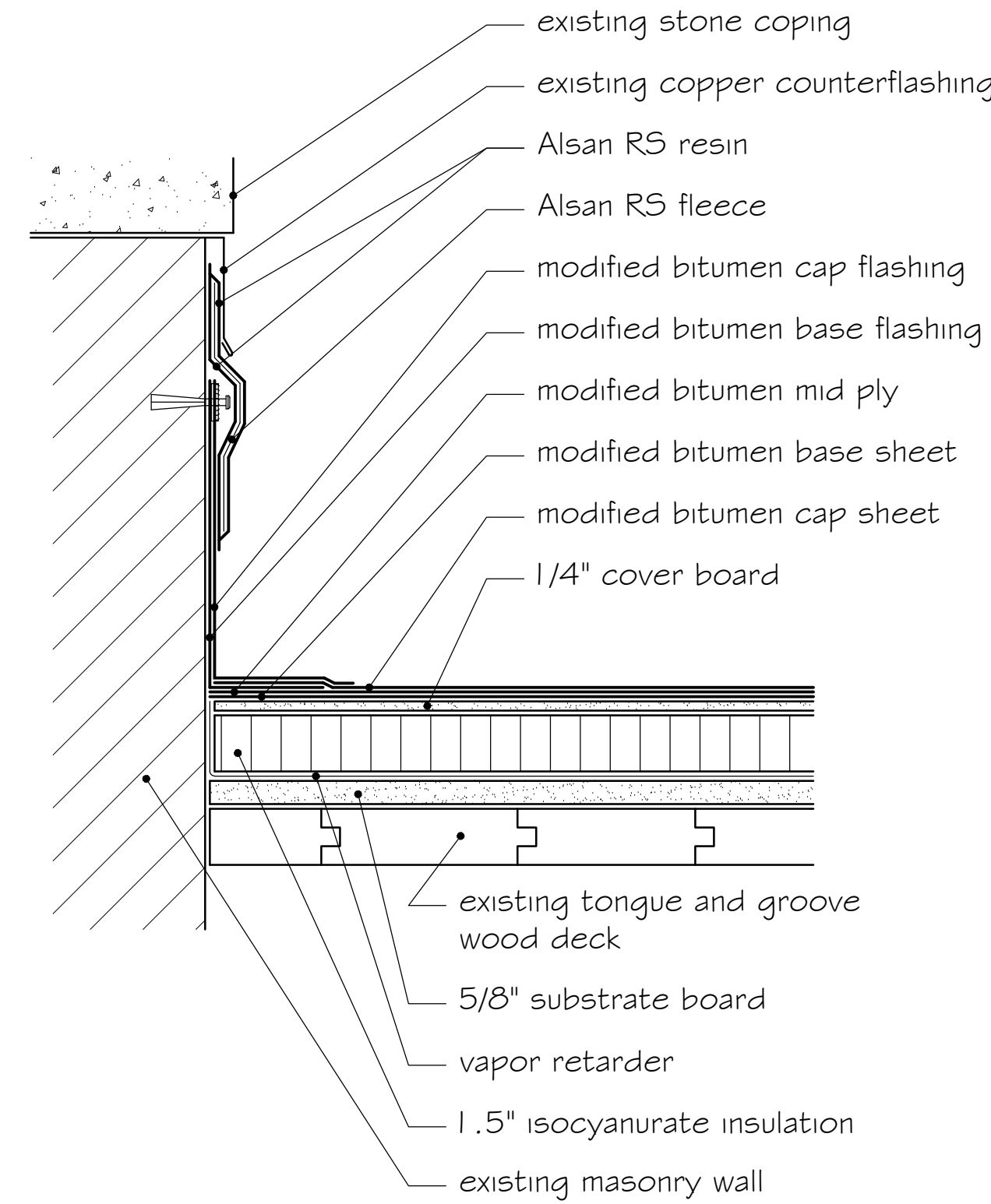
8 WALL FLASHING - AREA 29
