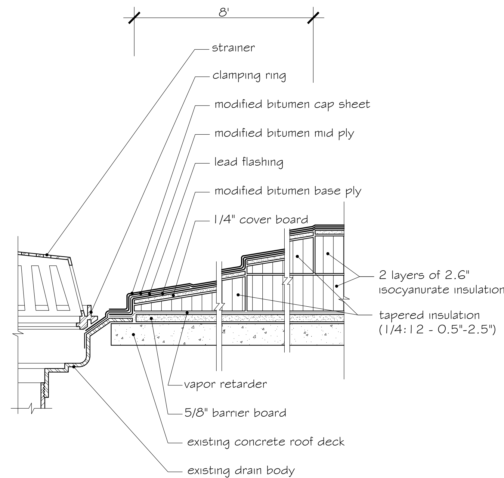
10 ROOF DRAIN - AREA 8
