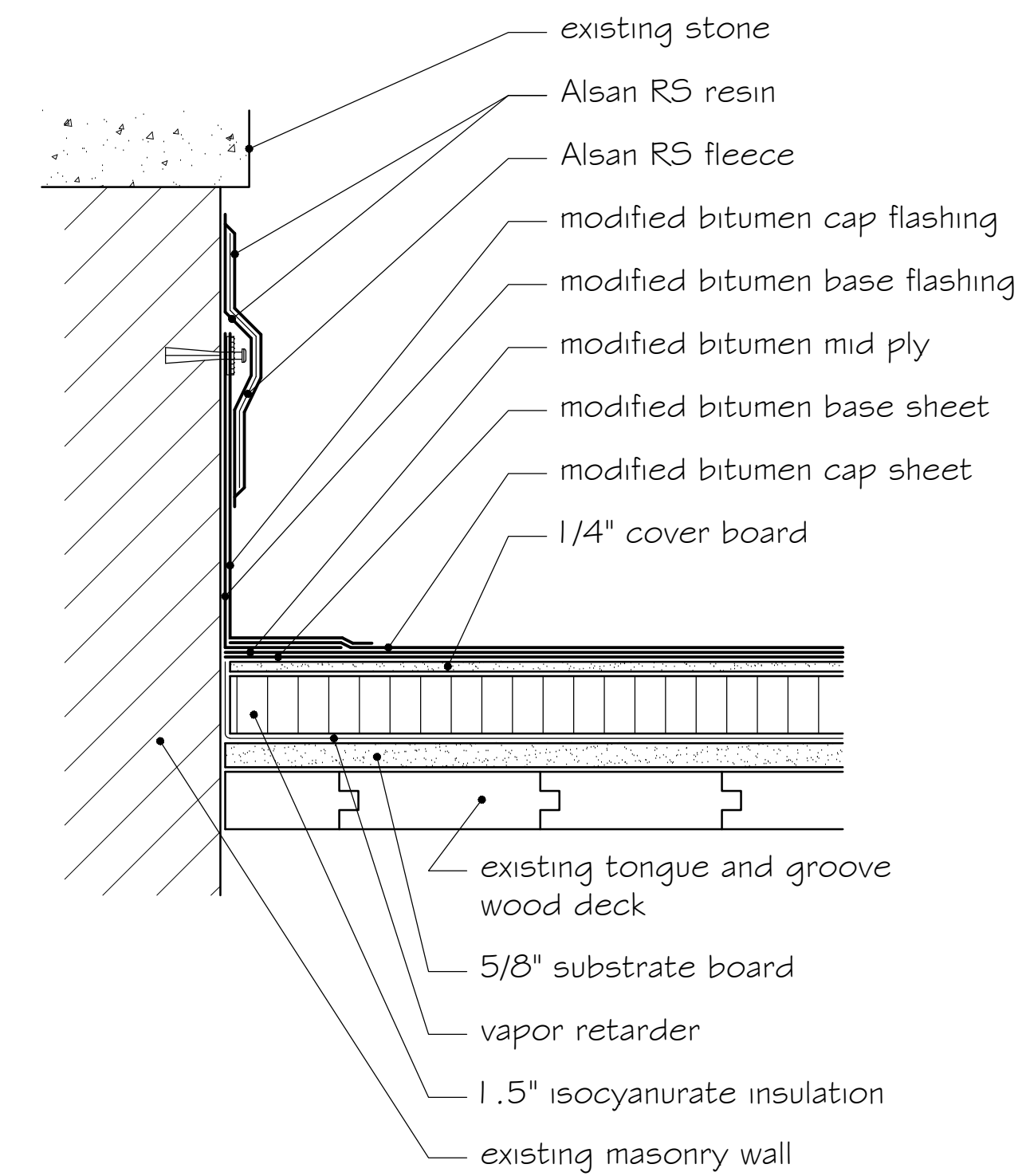
3 LIQUID APPLIED WALL TERMINATION - AREA 29 SCALE: 1" = 4"
