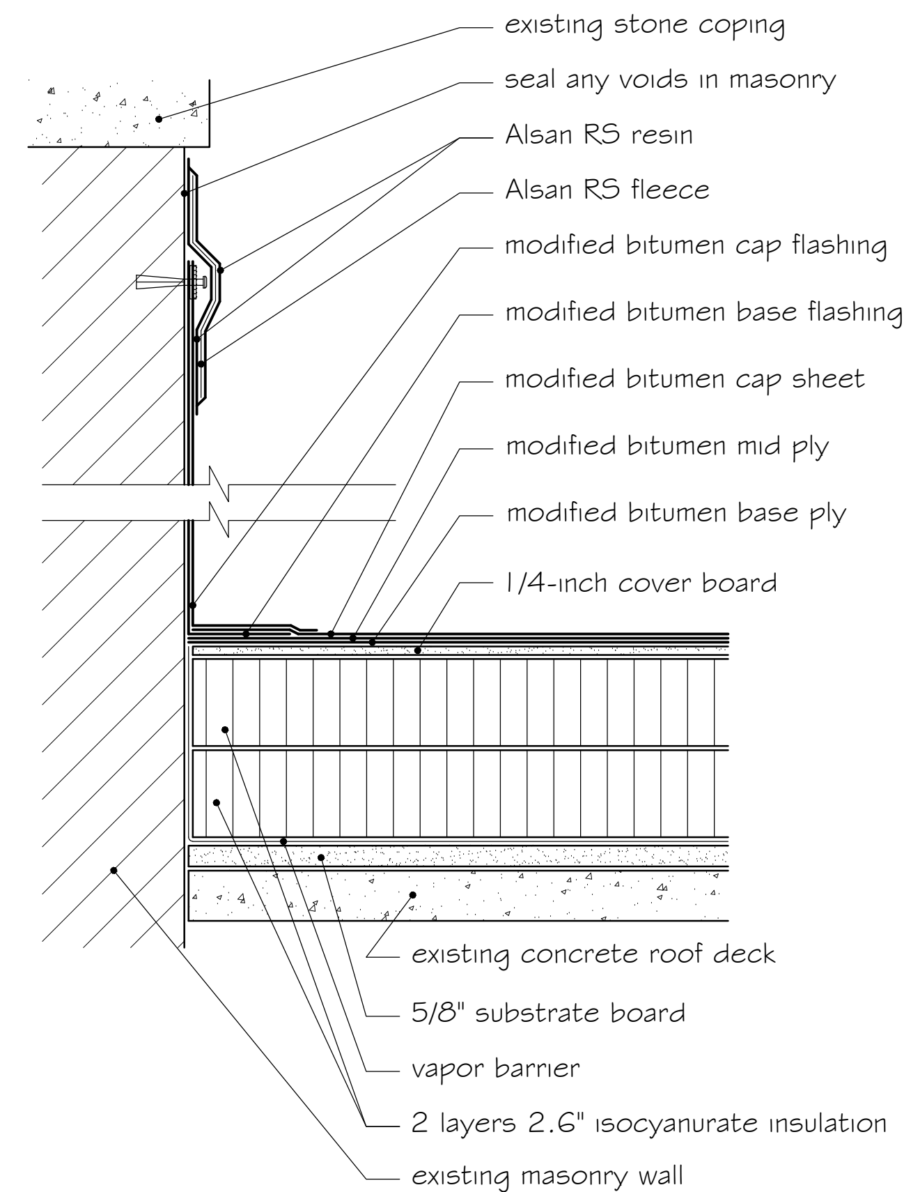
11 WALL FLASHING - AREA 8
