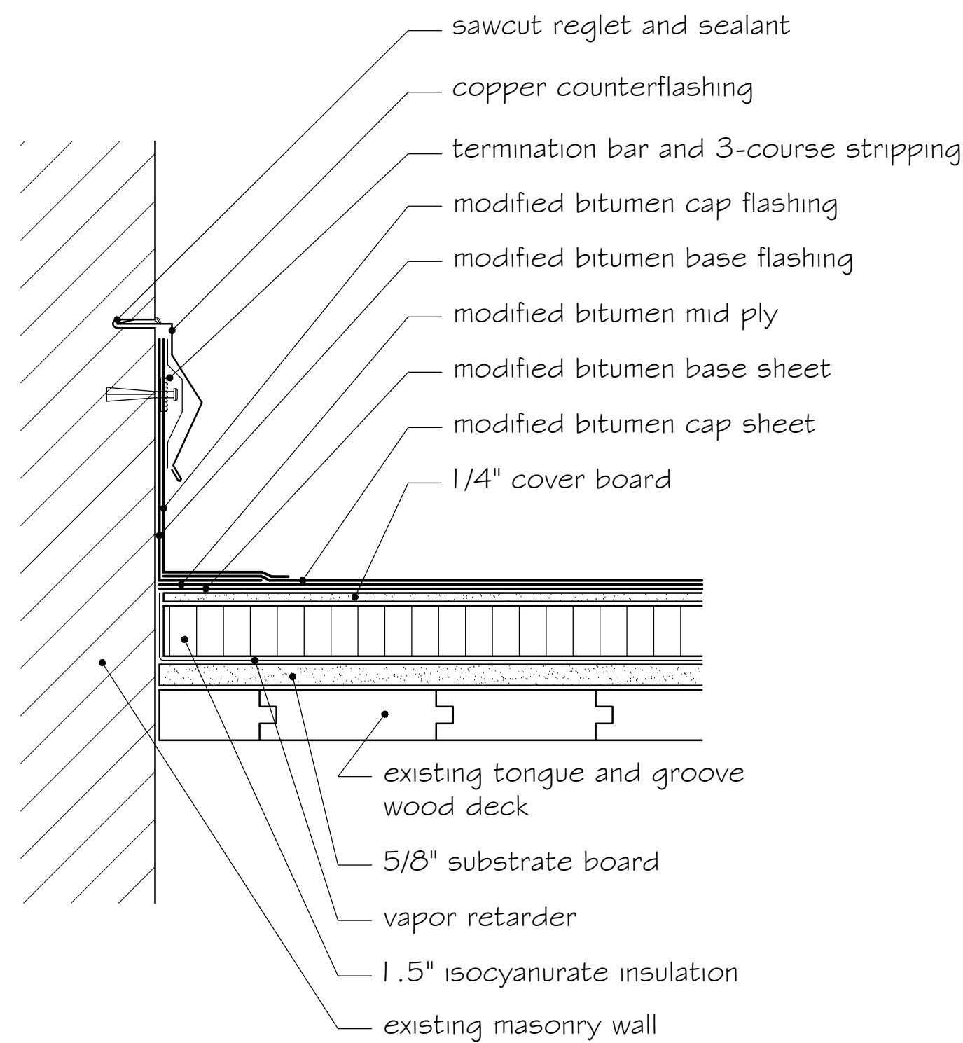
2 REGLET MOUNTED COUNTERFLASHING - AREA 29 SCALE: 1" = 4"
