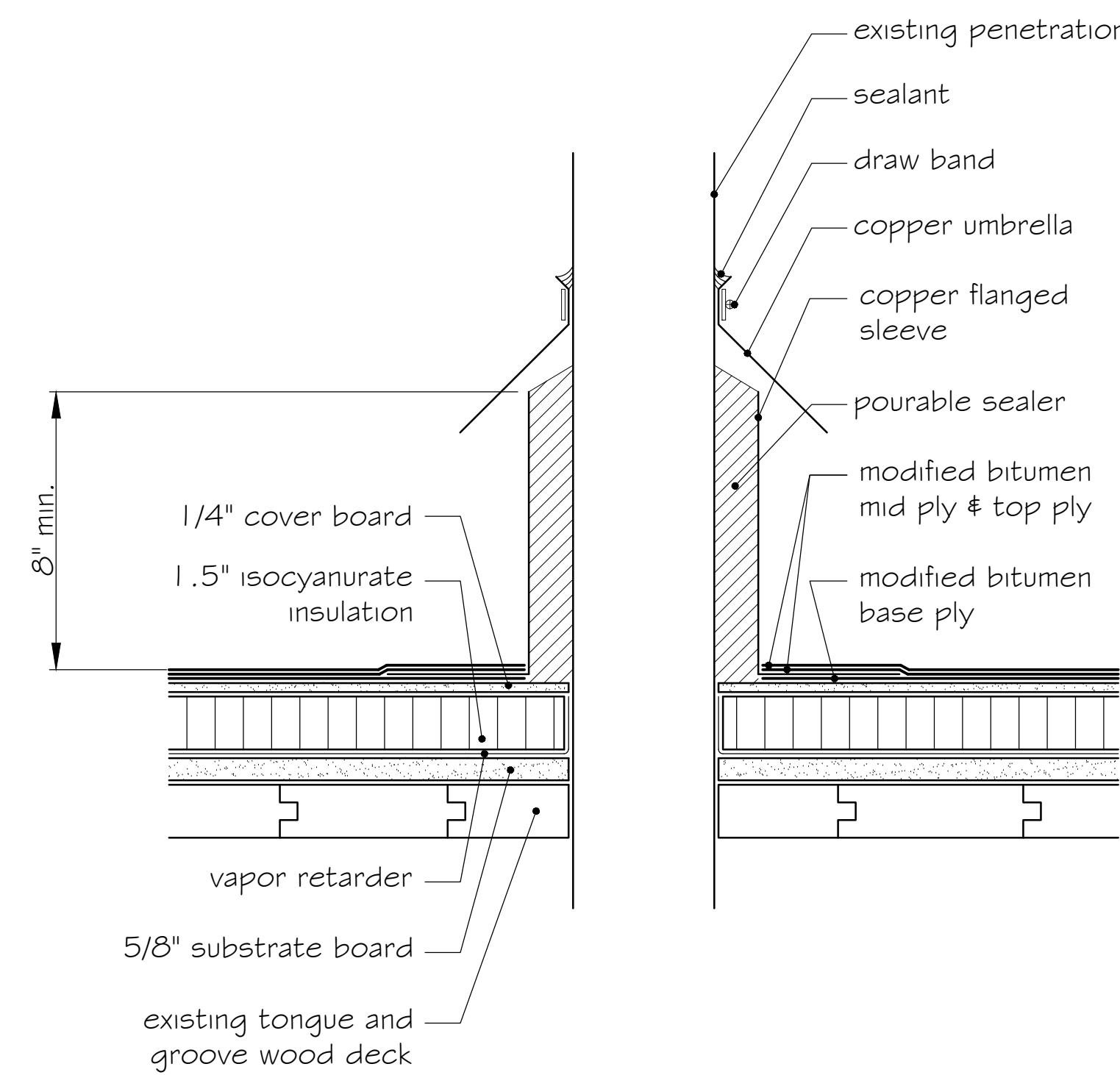
7 PLUMBING VENT PIPE FLASHING - AREA 29
