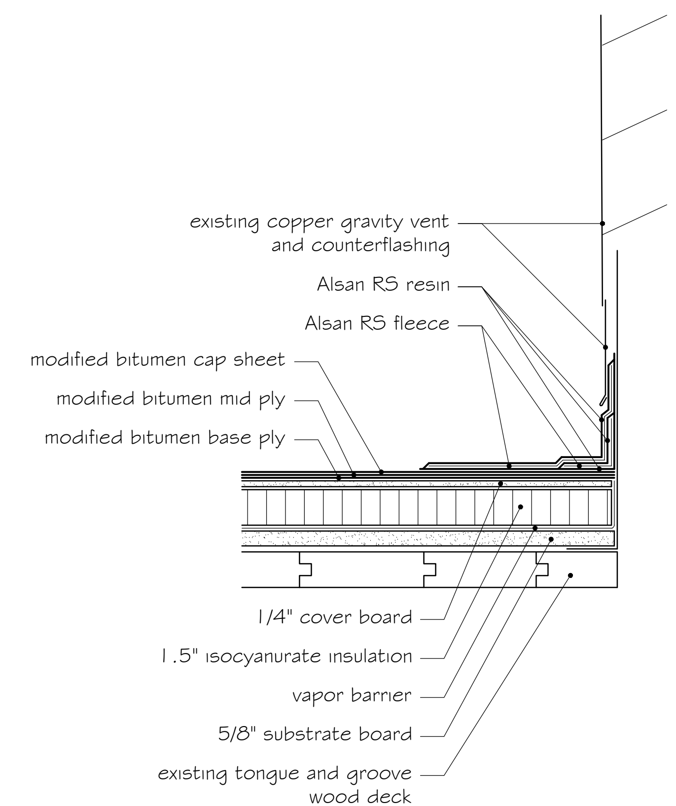
6 GRAVITY VENT FLASHING - AREA 29 SCALE: 1" = 4"
