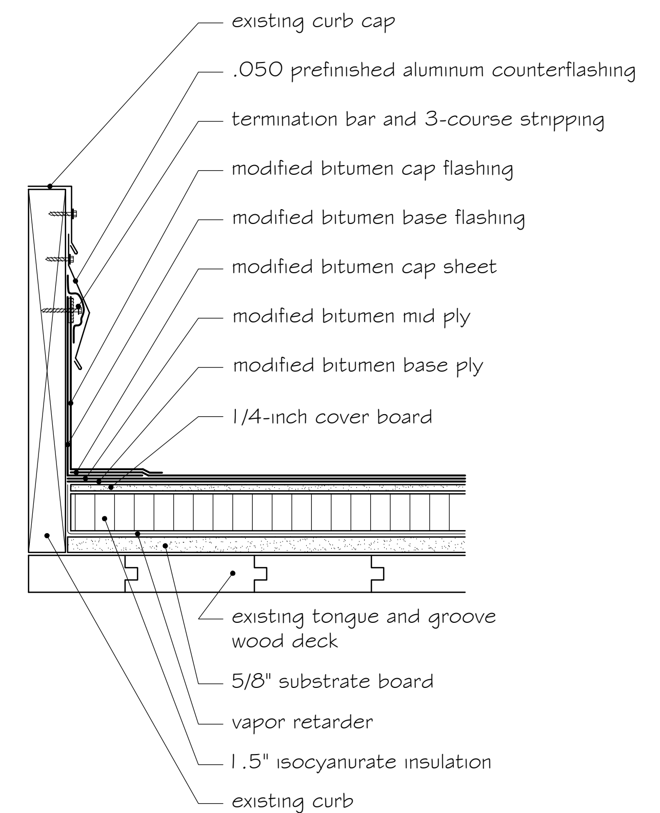
12 CURB FLASHING - AREA 29
