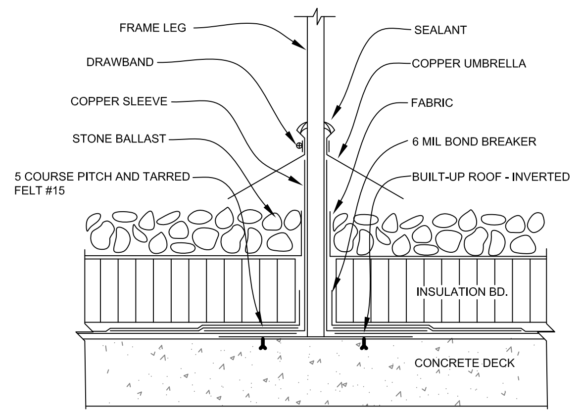
ELEVATED FRAME FLASHING NO SCALE
