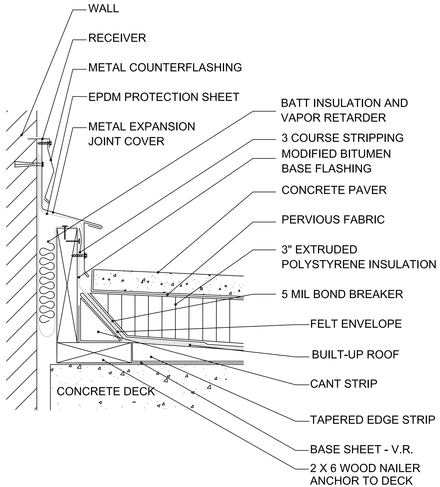
METAL WALL EXPANSION JOINT NO SCALE
