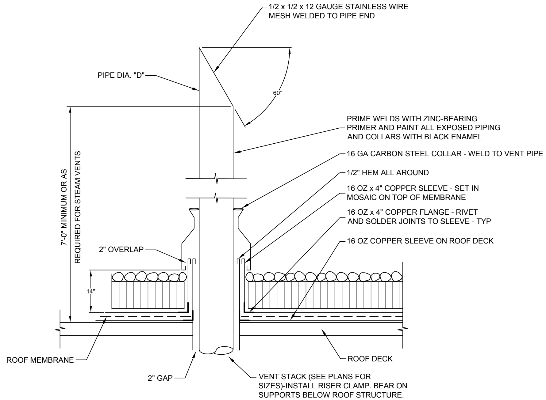
IRMA STEAM RELIEF VENT DETAIL NO SCALE
