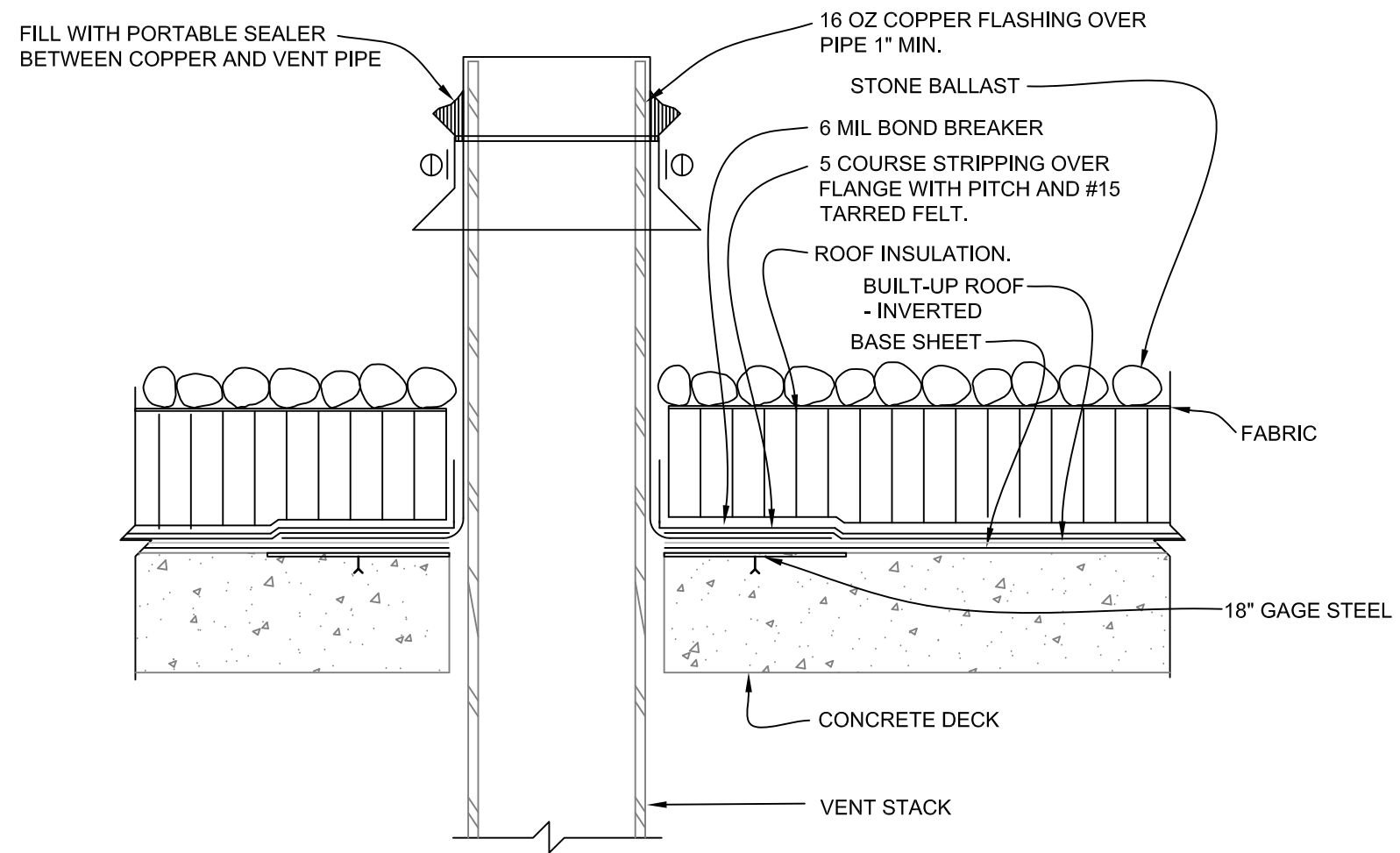
VENT STACK DETAIL NO SCALE
