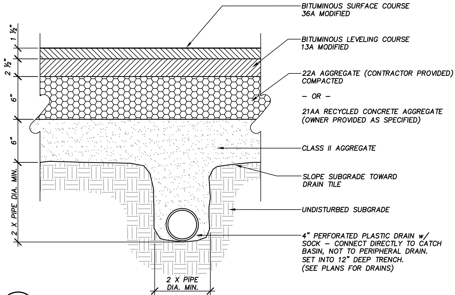
X X-X PARKING BITUMINOUS PAVEMENT SECTION SCALE: 1-1/2"=1'-0"
