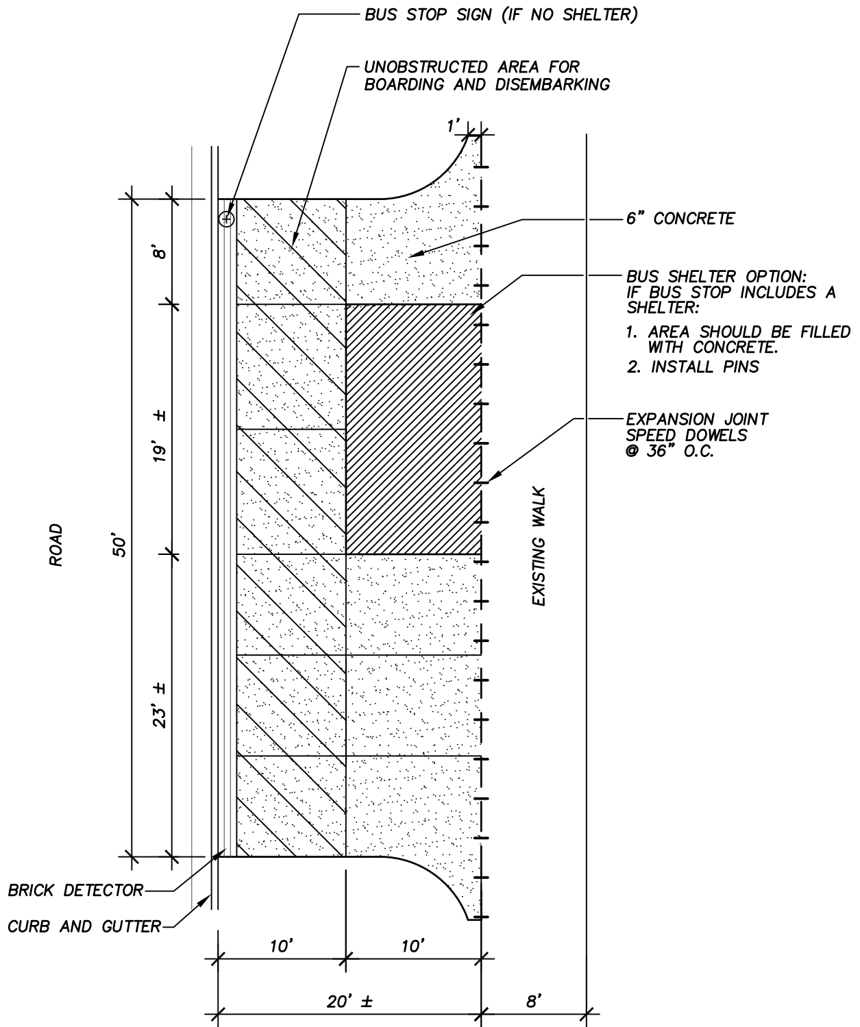
X X-X BUS STOP- NO CROSSWALK- HEAVY USE SCALE: 1" = 10'-0"
