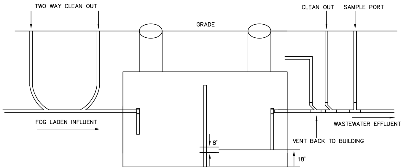
GREASE INTERCEPTOR TYPICAL DETAIL
