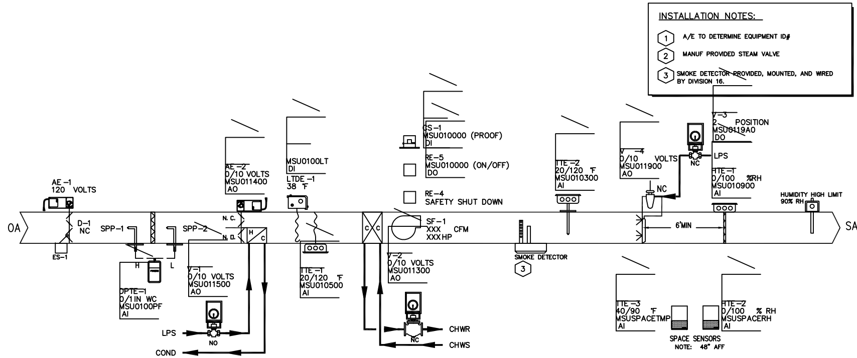
100% OA CONSTANT VOLUME AIR HANDLING UNIT WITH VIFB STEAM HEAT CONTROL DIAGRAM
