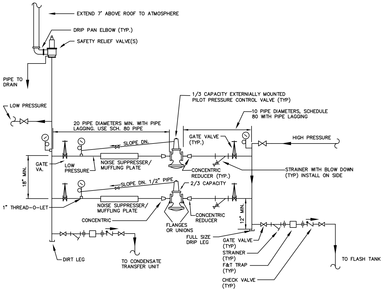
DUPLEX STEAM PRESSURE REDUCING STATION PIPING DETAIL NO SCALE
