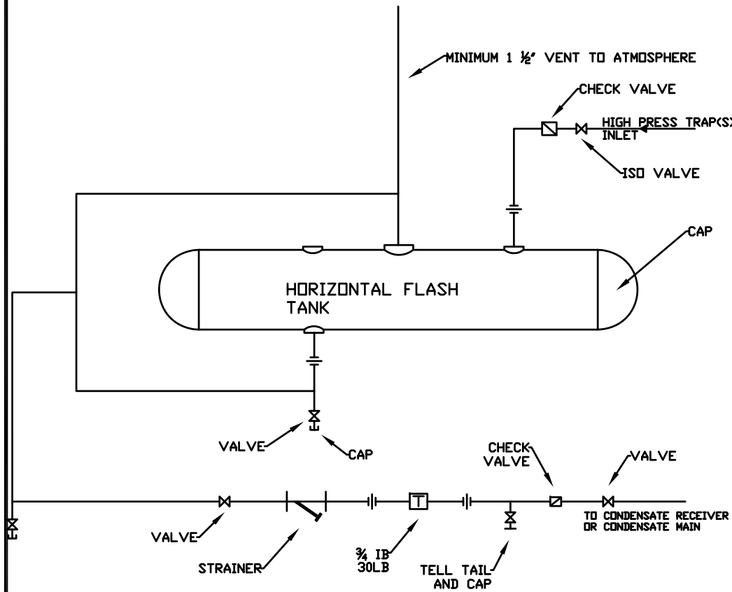
HORIZONTAL VENTED FLASH TANK
