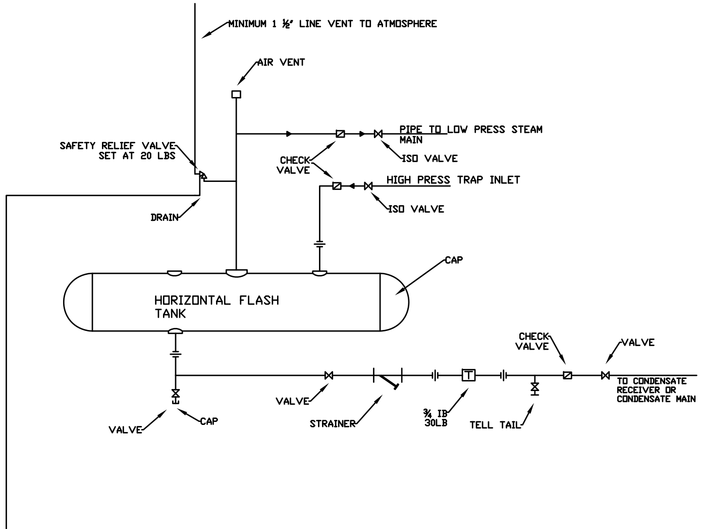
HORIZONTAL FLASH TANK WITH FLASH STEAM RECOVERY
