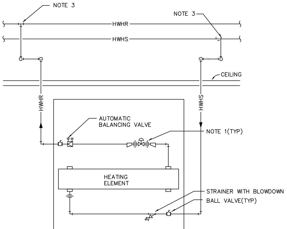
HWH CONVECTOR OR CABINET UNIT HEATER PIPING DIAGRAM WITH TWO-WAY CONTROL VALVE NO SCALE
