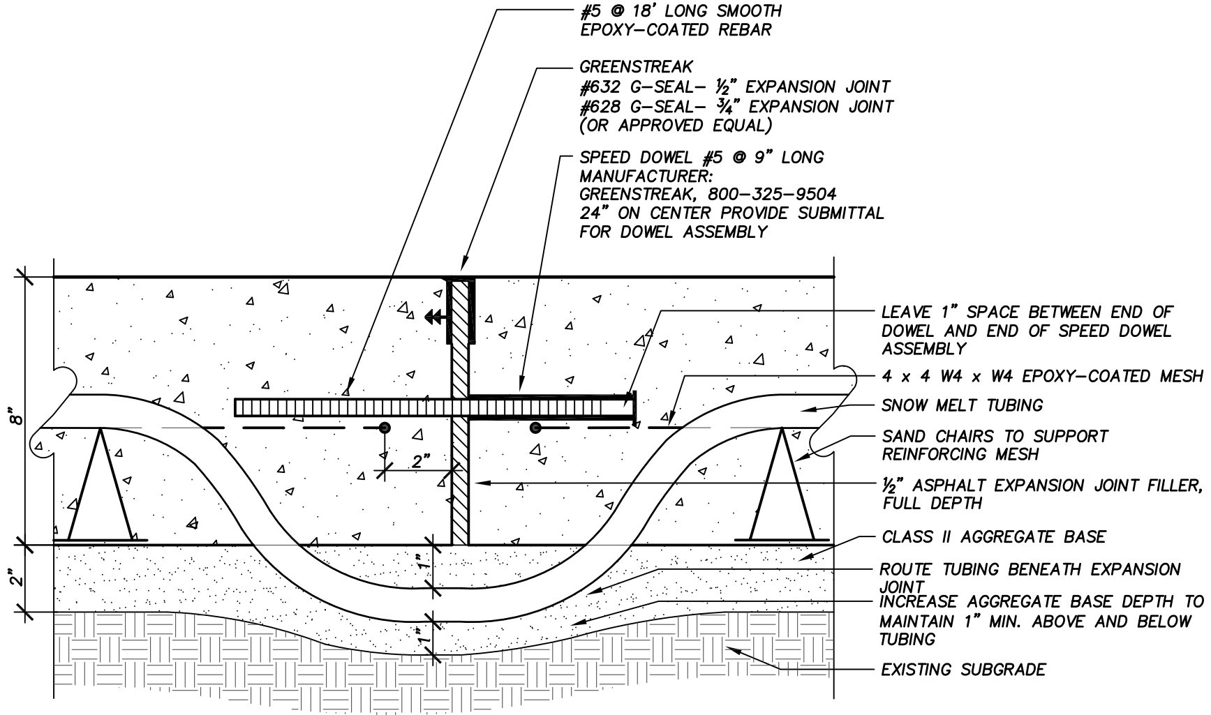
EXPANSION JOINT BETWEEN SNOW MELT ZONES Typical Detail
