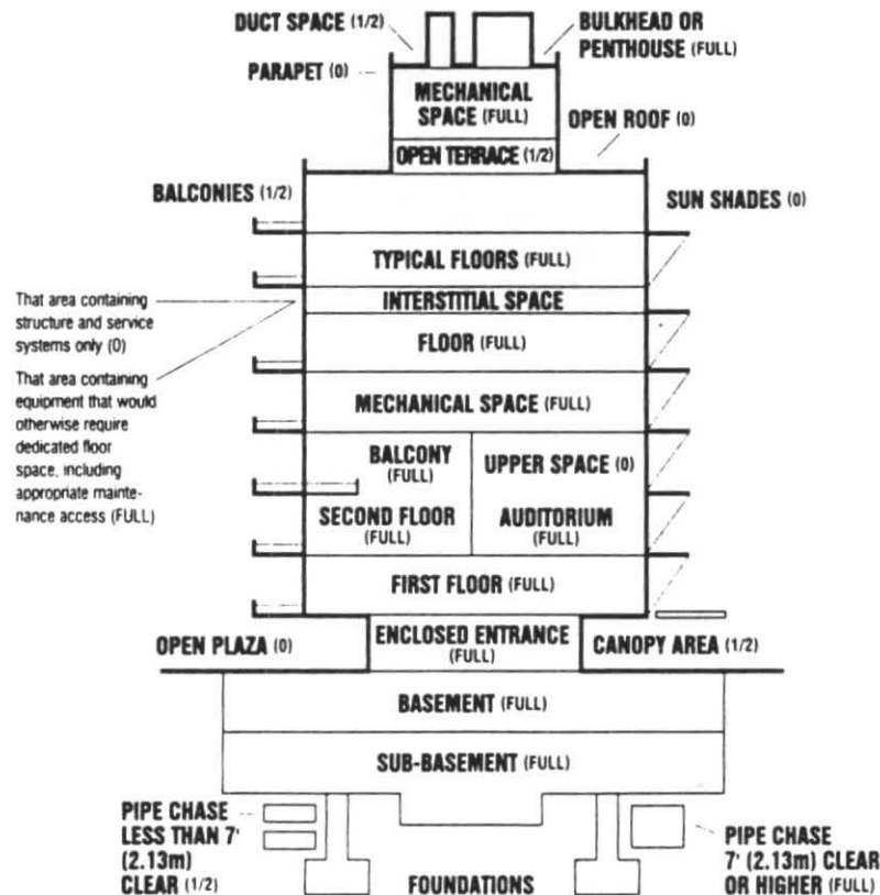
ARCHITECTURAL AREA DIAGRAM
