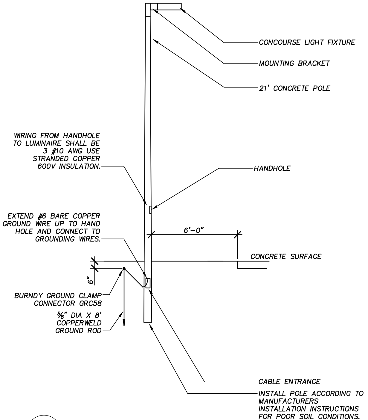
AREA LIGHT WITHOUT PULL BOX NOT TO SCALE
